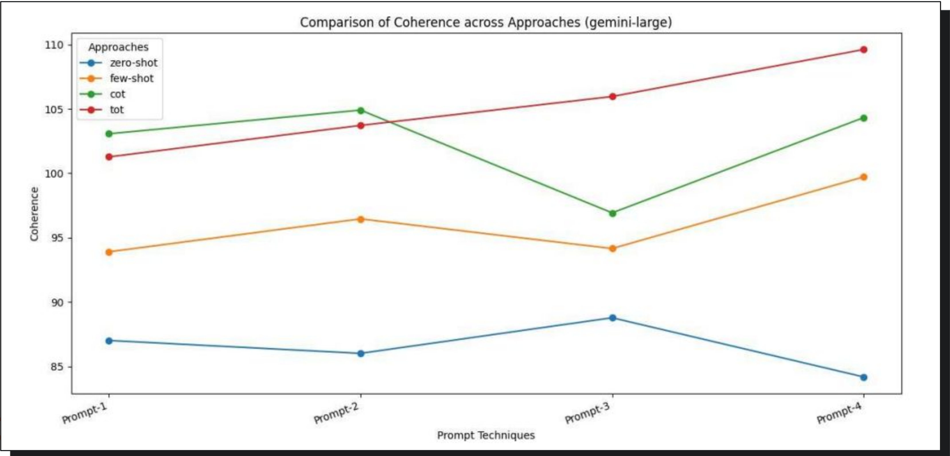
COMPARISON OF COHERENCE OF GEMINI-LARGE MODEL WITH DIFFERENT PROMPTS
