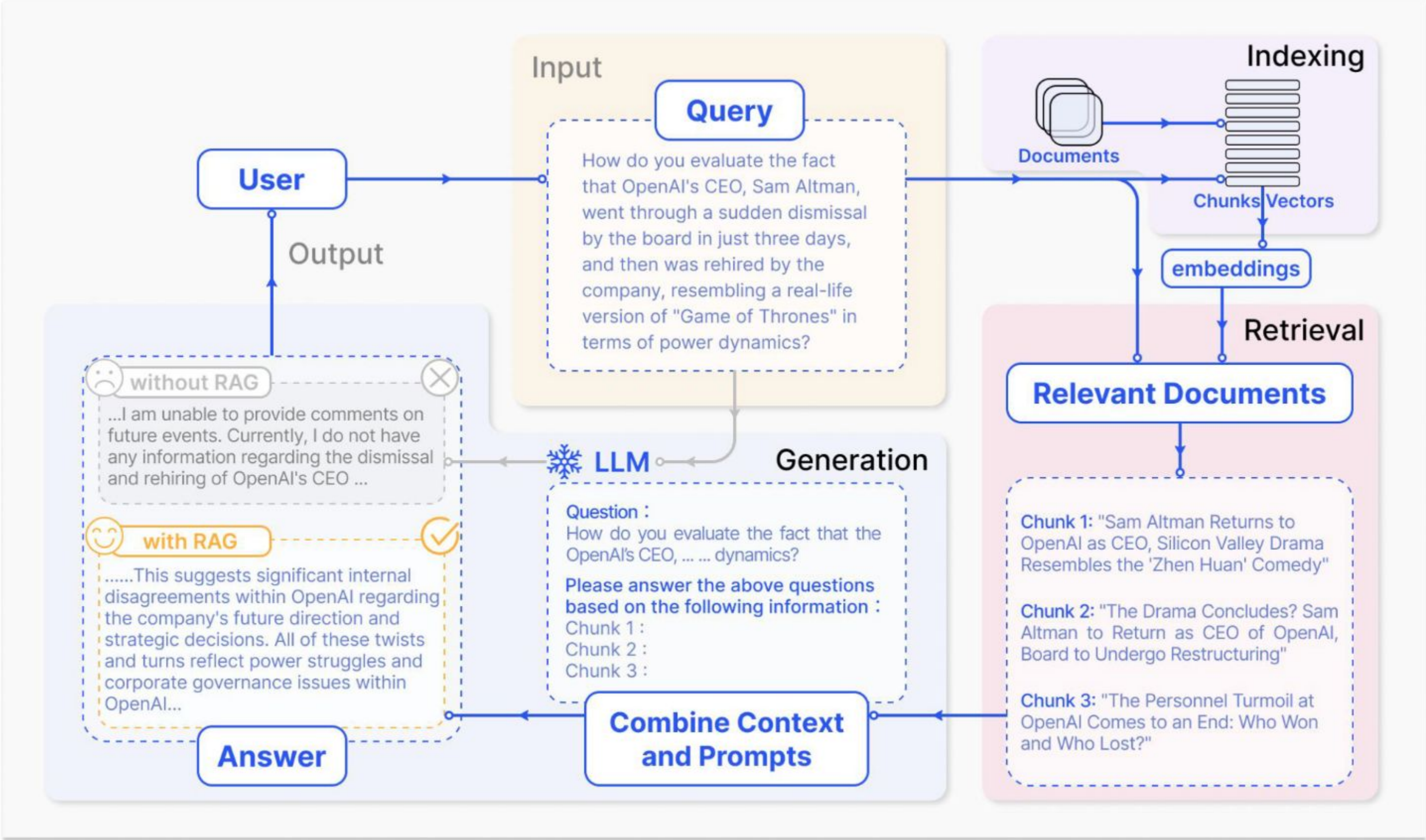
A typical case of RAG
