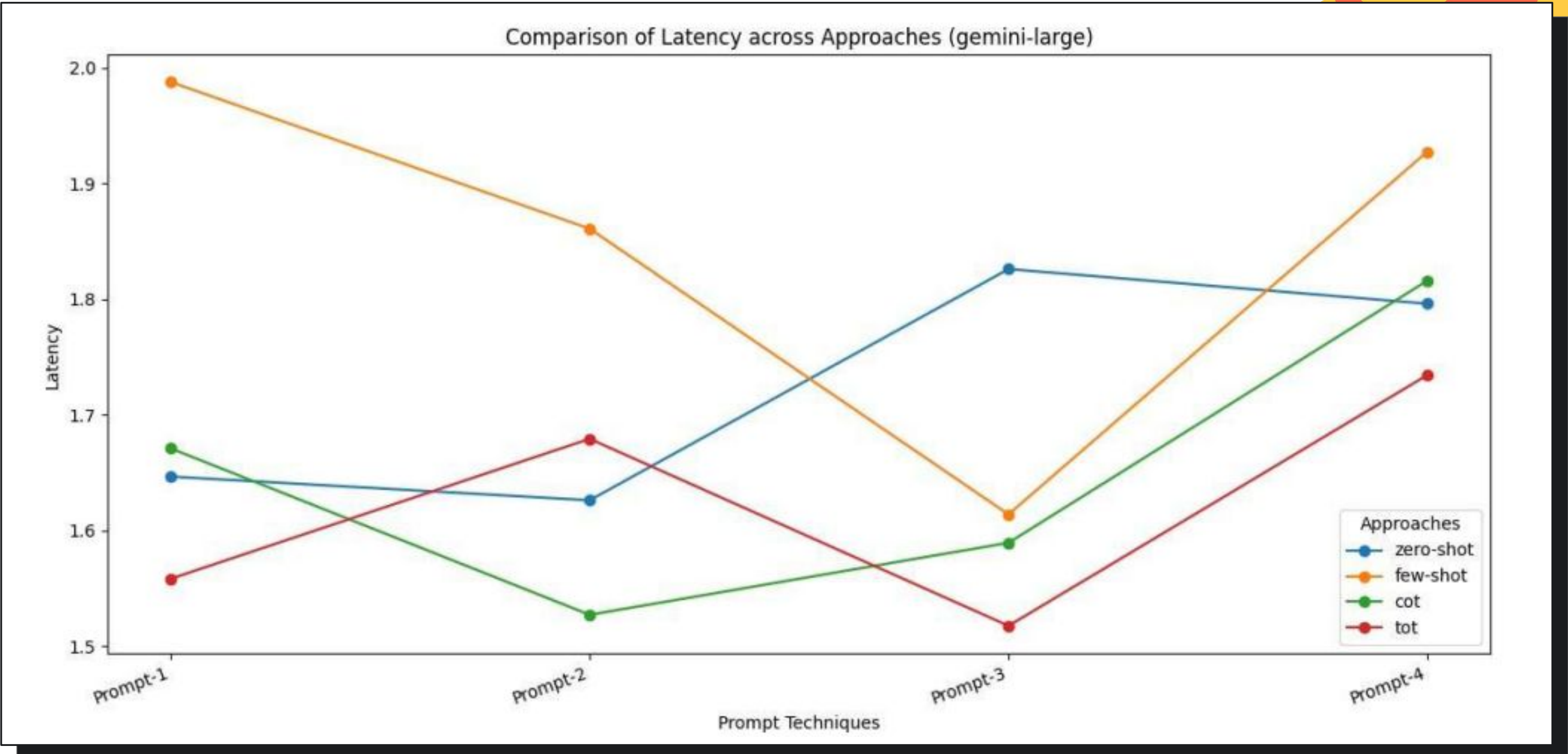
COMPARISON OF LATENCY OF GEMINI-LARGE MODEL WITH DIFFERENT PROMPTS
