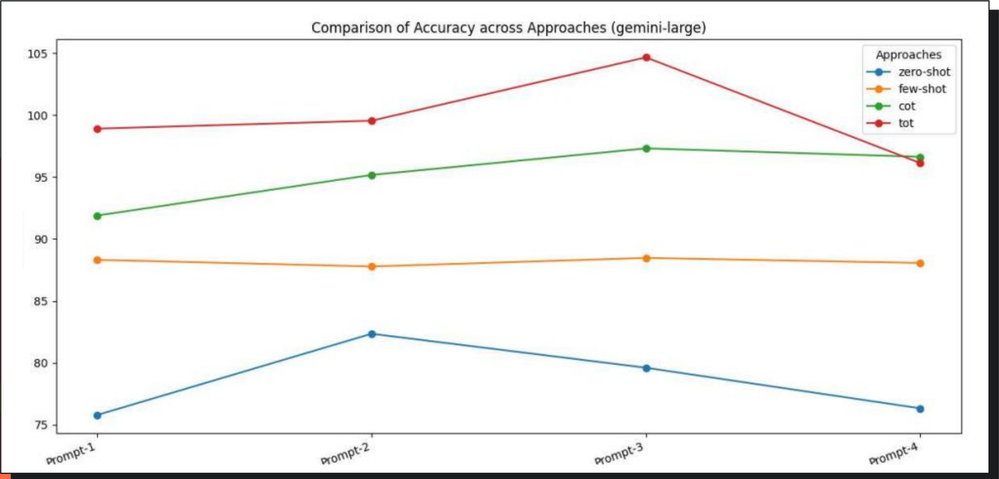
COMPARISON OF ACCURACY OF GEMINI-LARGE MODEL WITH DIFFERENT PROMPTS
